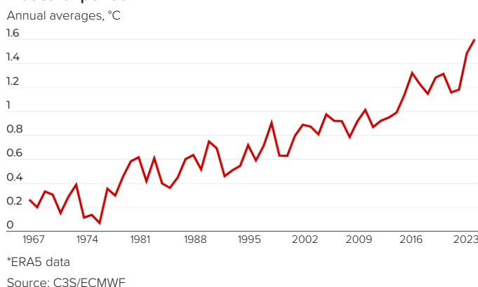
CHART 12: Global surface temperature increase above pre-industrial period*
