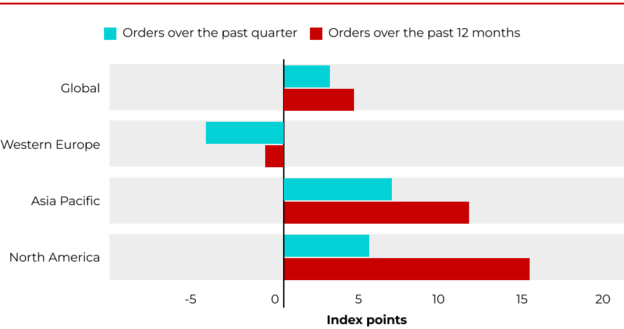
Chart 9 Change in the GECS New Orders index, by region*
